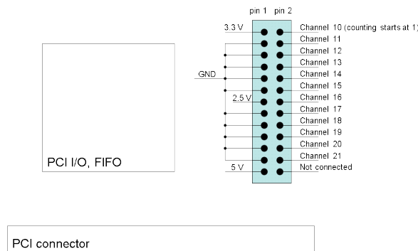
Figure 1.3: LowRes Pinout
